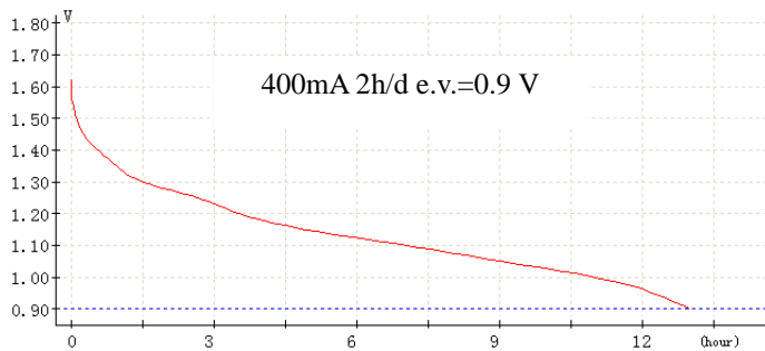
Chart 1. Discharge diagram
