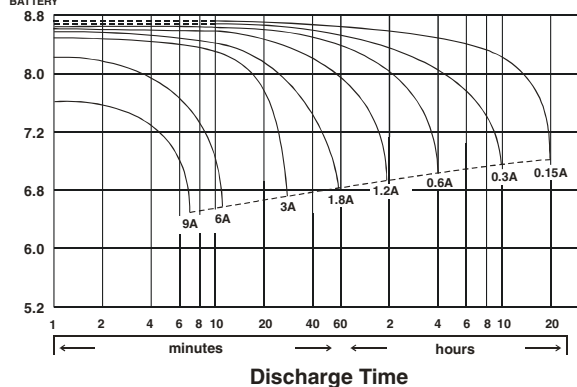
(V) FOR 8V BATTERY Discharge Time VS. Discharge Current (25°C)
